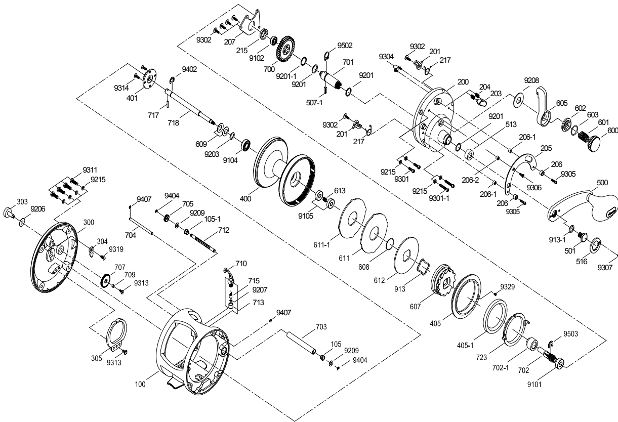
TG - 10L (1 of 2) Spare Parts
